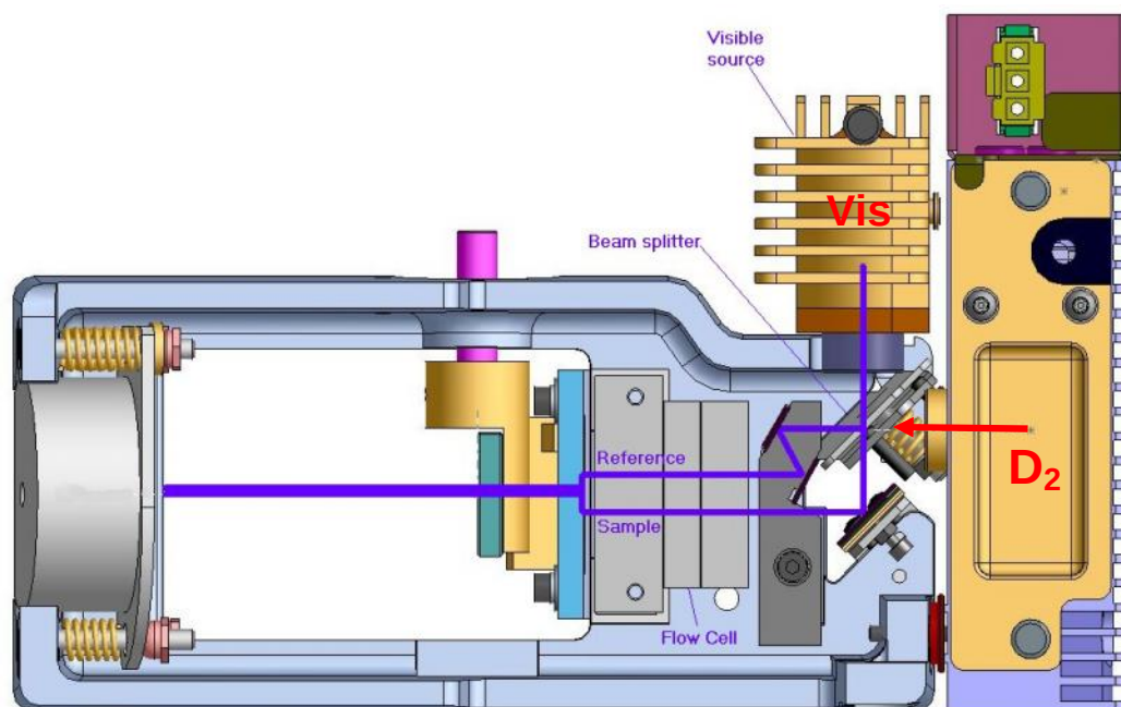
Visible lamp light path (in purple)
