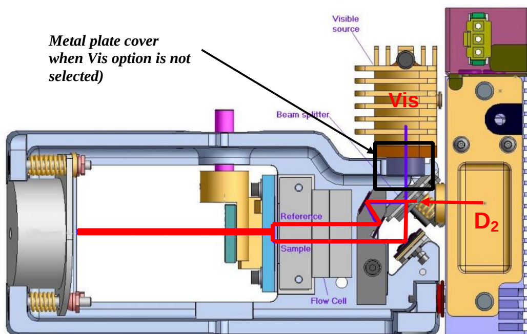
UV (D 2 ) lamp light path (in red)
